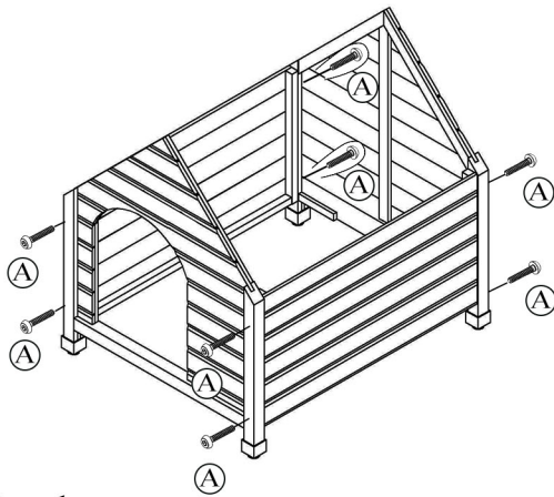
Step 1: Secure side panels with bolts
