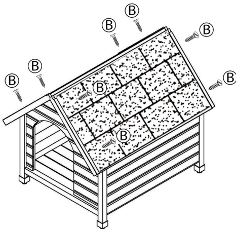
Step 3: Attach roofs and secure with screws
